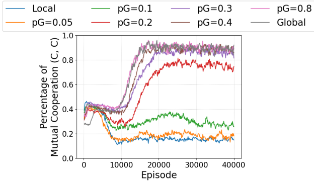
Figure 2: The percentage of mutual cooperation (C, C) across episodes with agents acting based on different probabilities p_G of utilising global information. The cooperation rate rises with p_G . Local means p_G = 0 and Global p_G = 1 .
